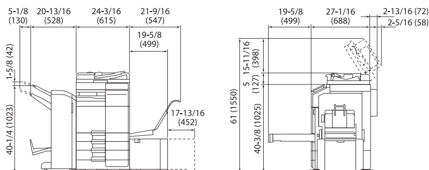
Main unit + DF-632 + FS-536 SD + PC-216 + LU-302 + MK-730 + CU-102
