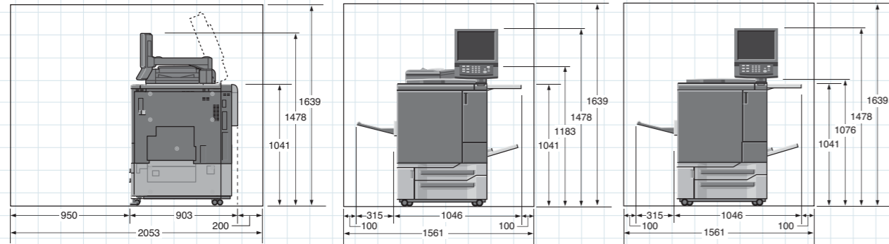
Side View bizhub PRESS C1070/C1060+OT-502+ DF-626+MB-506
